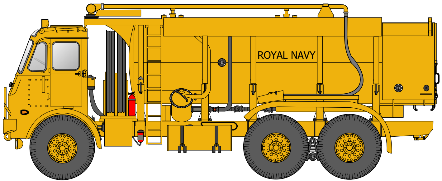
Leyland Hippo Mk.2/3 Airfield Refueller - Royal Navy RNAS Yeovilton 1970's-80's BS381C 356 Golden Yellow
