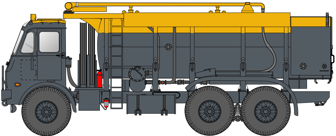
Leyland Hippo Mk.2/3 Airfield Refueller - RAF Cottesmore, 1960's BS381C 633 RAF Blue-Grey and BS381C 356 Golden Yellow
