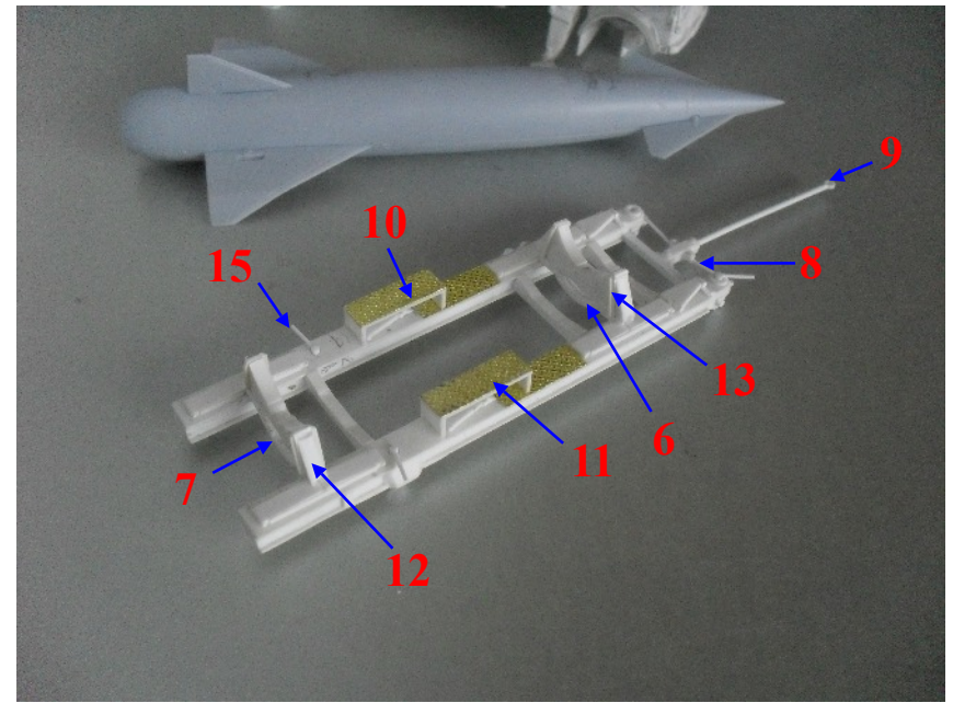
Stage 3: Fit towing arm bogey Part 8 and towing arm Part 9. Note position of cross frames Part 6 and 7 under the missile cradles Parts 12 & 13.
