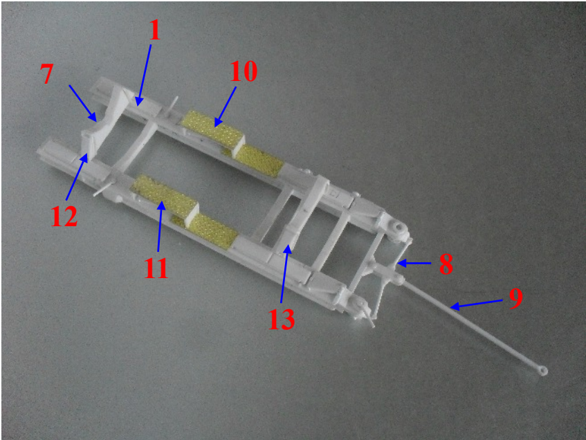
Stage 2: Fit working platforms 10 and 11, cross frame Part 7 & missile cradles Part 12 and 13.
