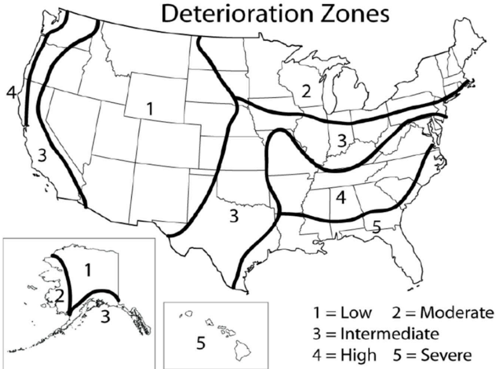
Figure 4. Current AWPA fungal decay hazard map from the 2016 AWPA Book of Standards.
