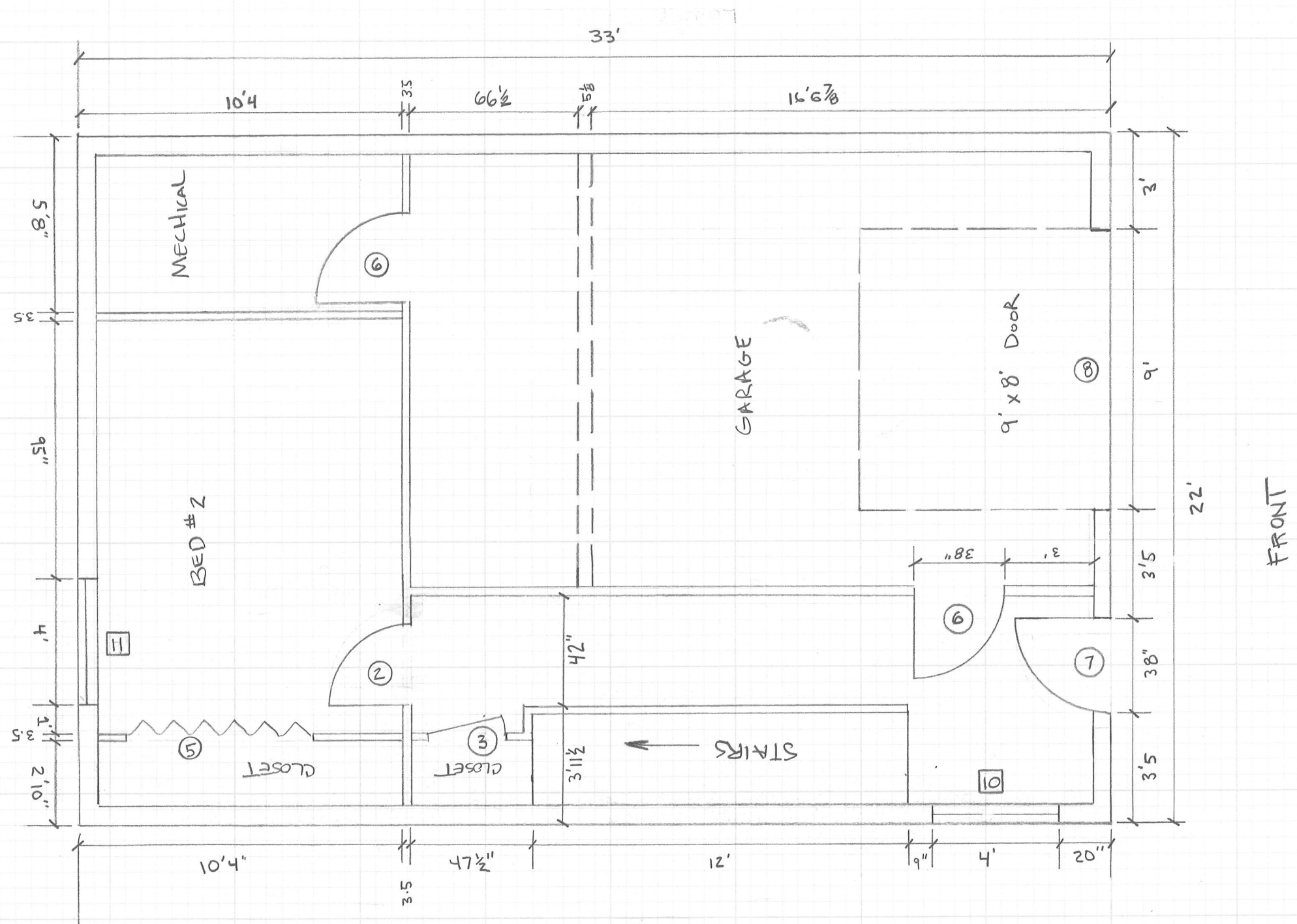
LOWER LEVEL FLOOR PLAN
