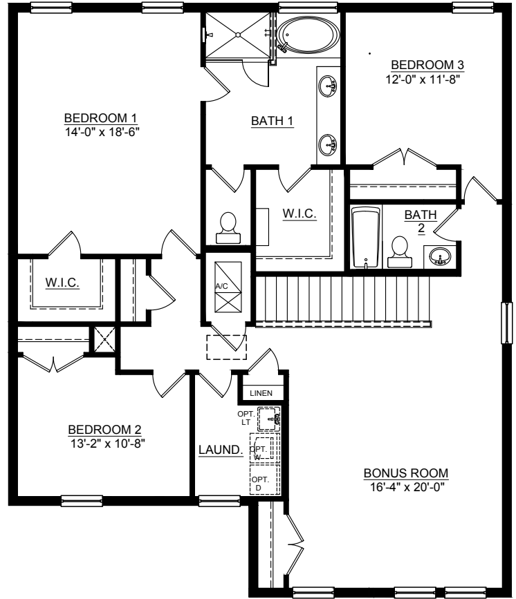
Second Floor Plan - Elevation G & H
