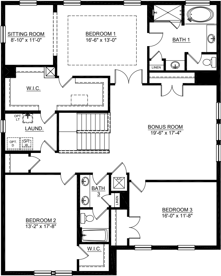
Second Floor - G & H
