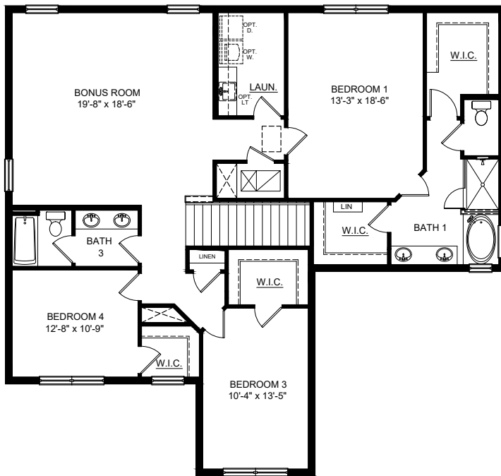
Second Floor - Elevation G & H
