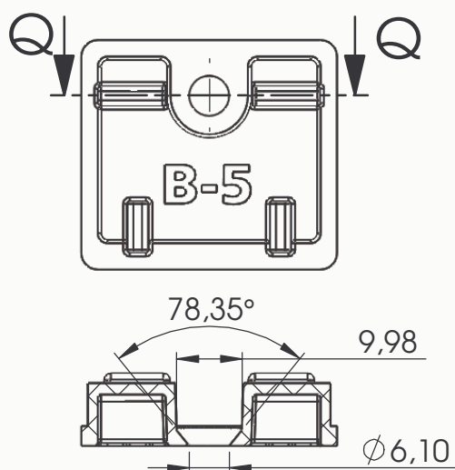
SECTION Q-Q SCALE 1 : 1
