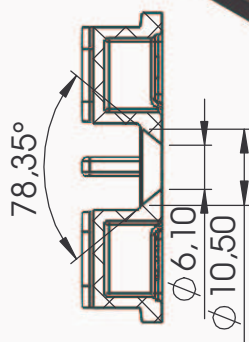
SECTION H-H SCALE 1 : 1
