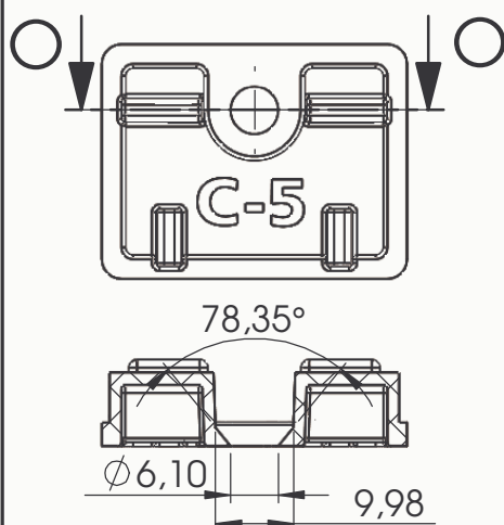
SECTION O-O SCALE 1 : 1
