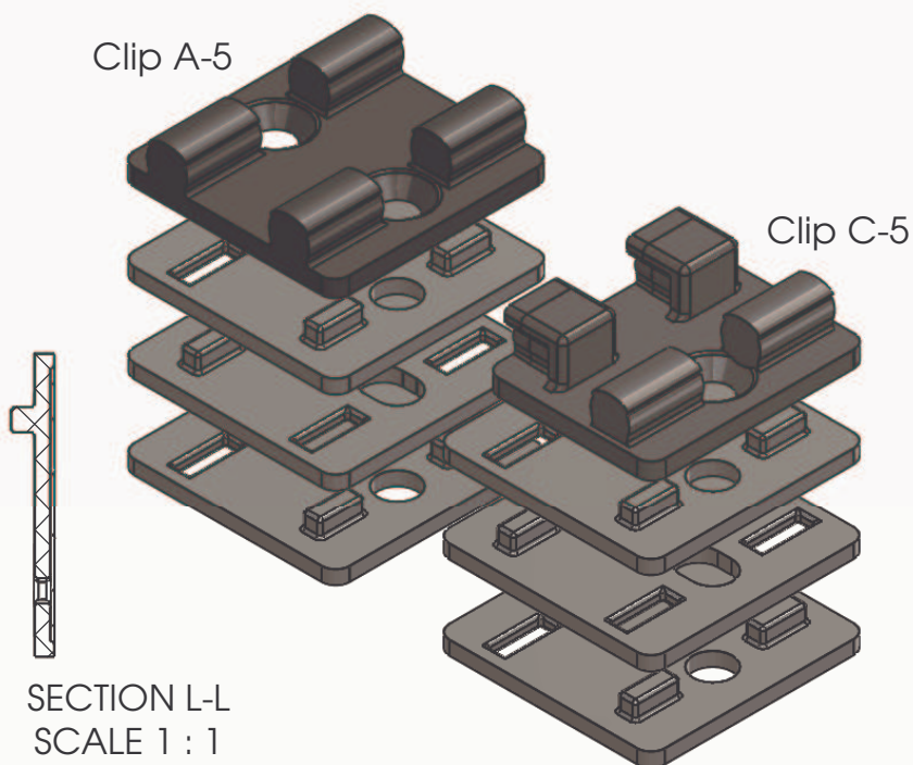
Exploded view: Spacer A-C 5 (6pc.)
