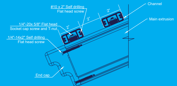
TRELLIS, DETAIL A
