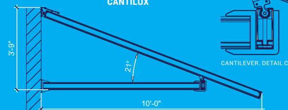
CANTILEVER, MAX ANGLE
