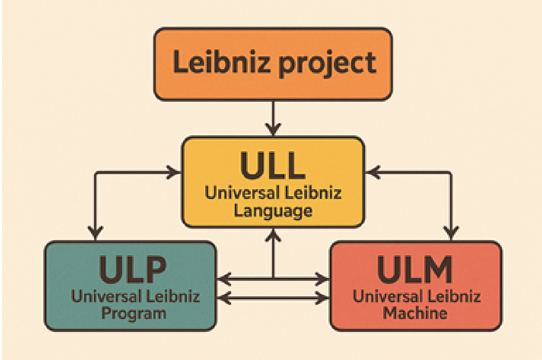
FIGURE 2. LP interconnections via Centrics-formulated “arrows”
