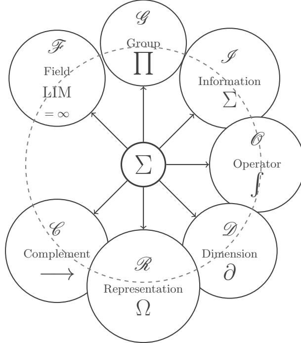
Septenary (Heptad)-Trialic Regime of the Centrics Operator
