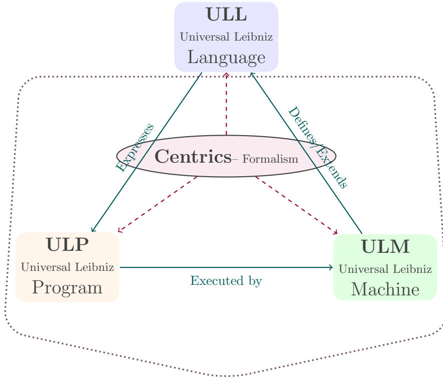
Leibniz Project Triad (Centrics Formulation)
