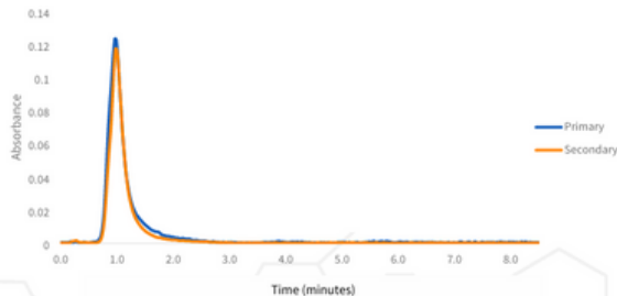
Chromatogram
