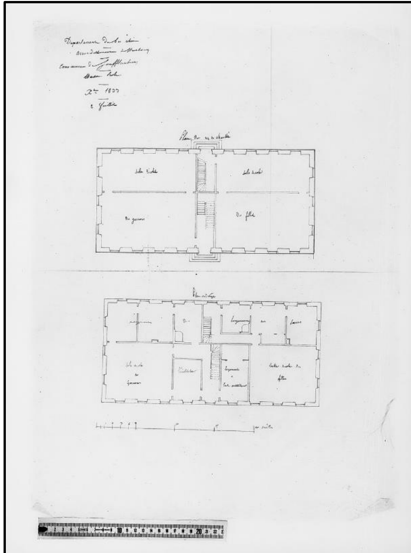
Soufflenheim School Plan, 1833
