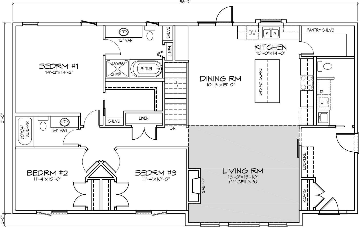
FLOOR PLAN #1706 1777 SQ. FT.
