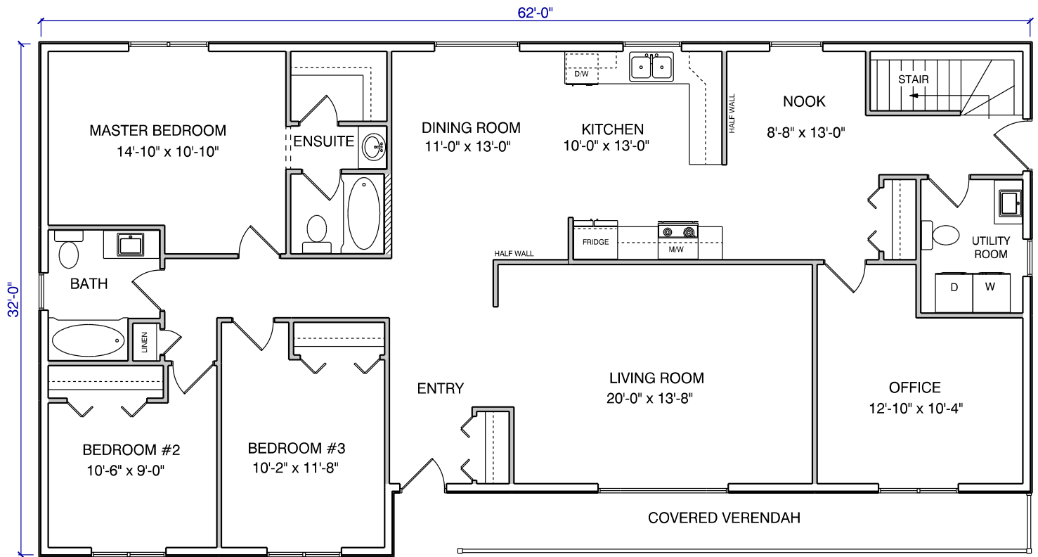
FLOOR PLAN #1801
