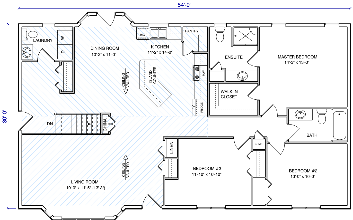
FLOOR PLAN #1607 1651 SQ. FT.
