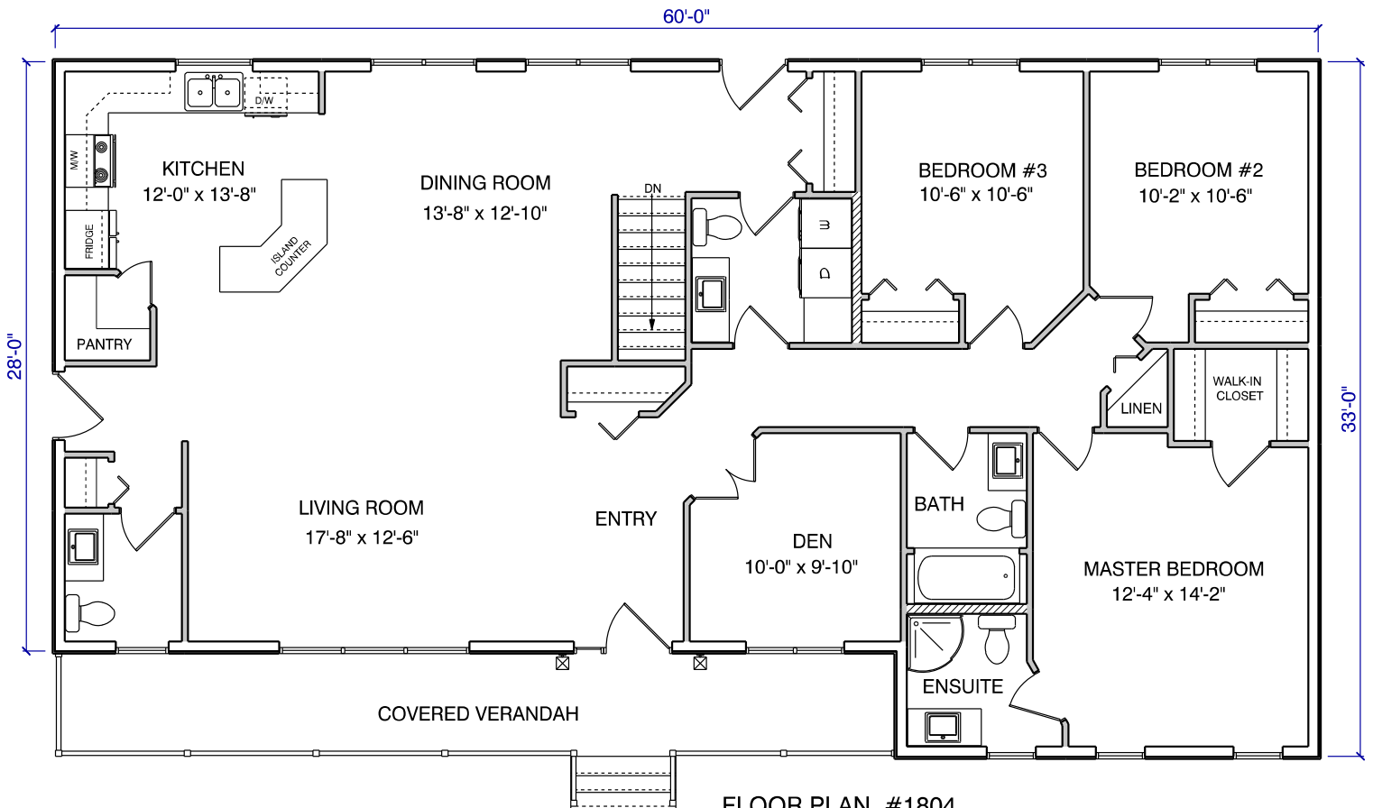
FLOOR PLAN #1804
