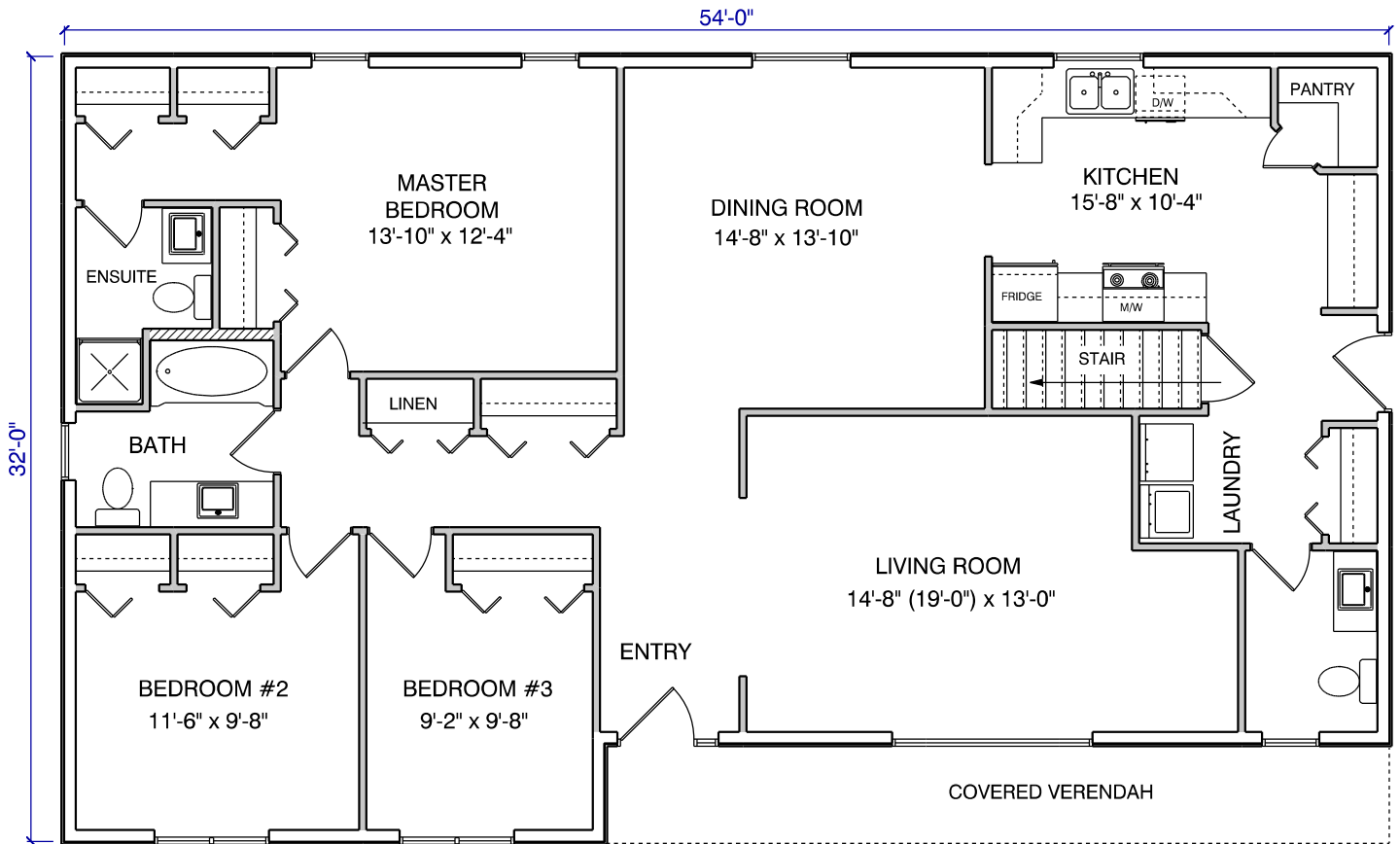
FLOOR PLAN #1603
