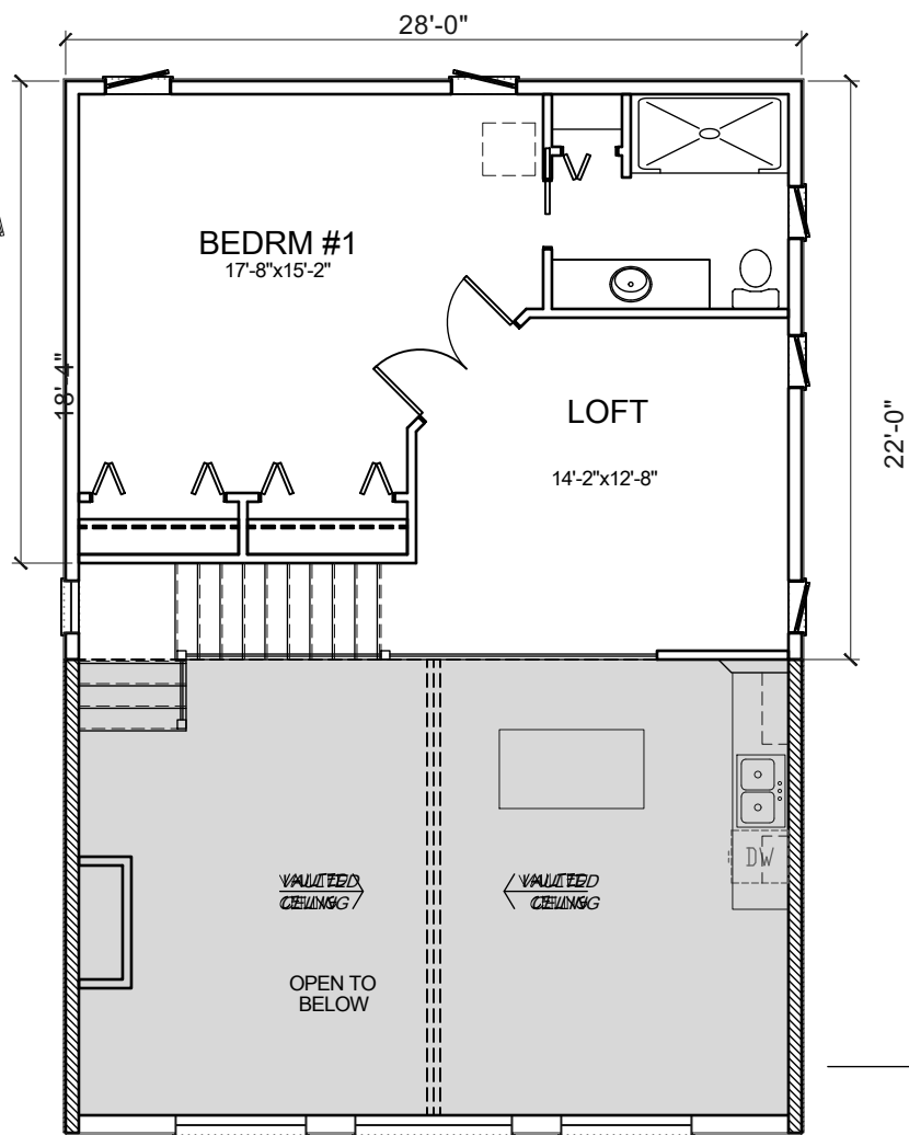
UPPER FLOOR PLAN #1615 572 SQ. FT.
