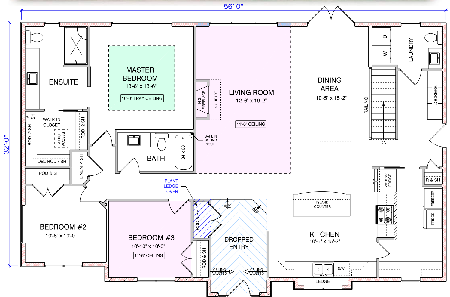
FLOOR PLAN #1903 1906 SQ. FT.
