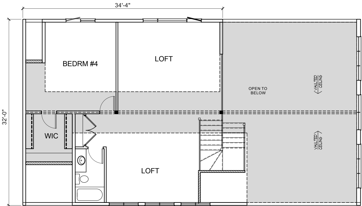
UPPER FLOOR PLAN #2800
