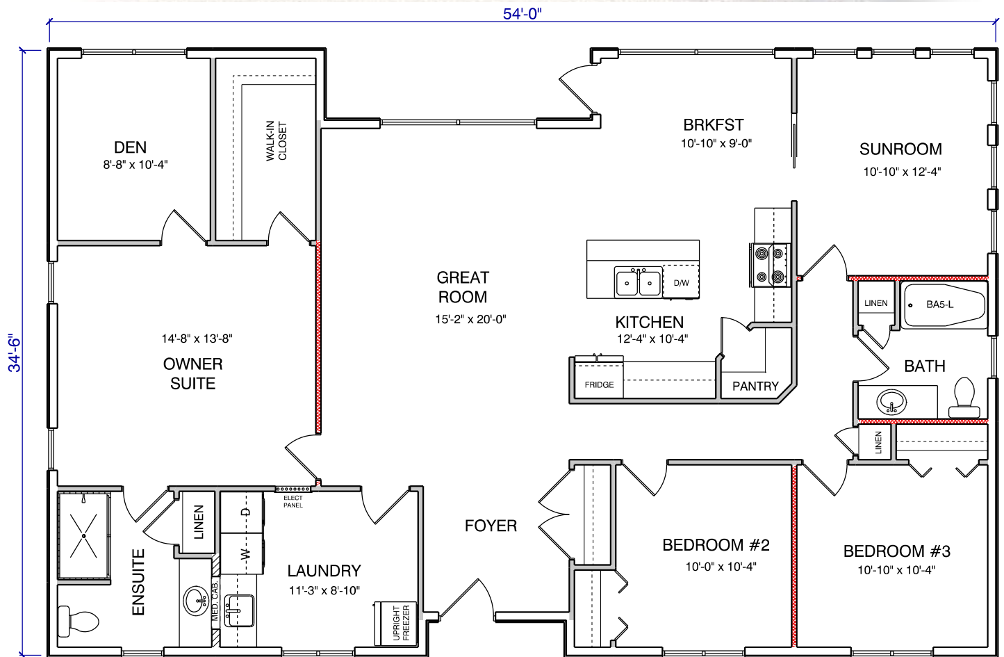
FLOOR PLAN #1700 1787 SQ. FT.
