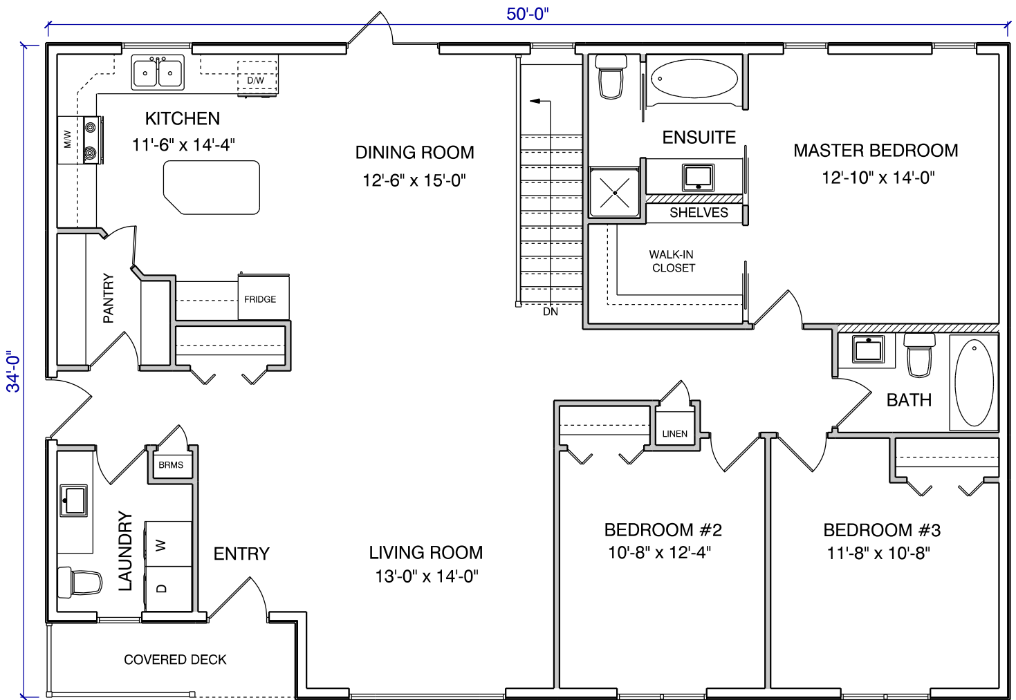
FLOOR PLAN #1606 1648 SQ. FT.
