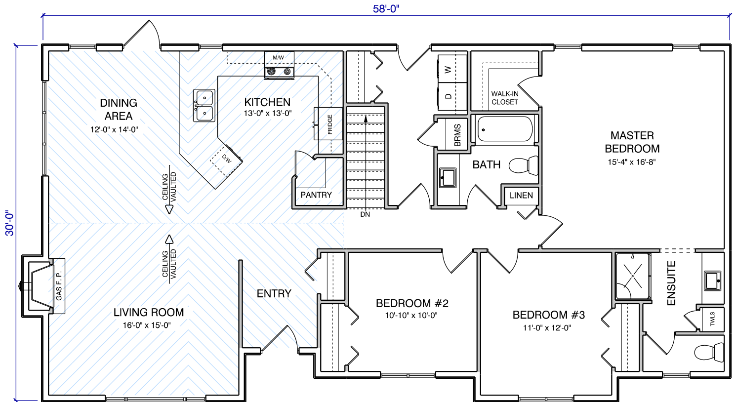
FLOOR PLAN #1611 1678 SQ. FT.
