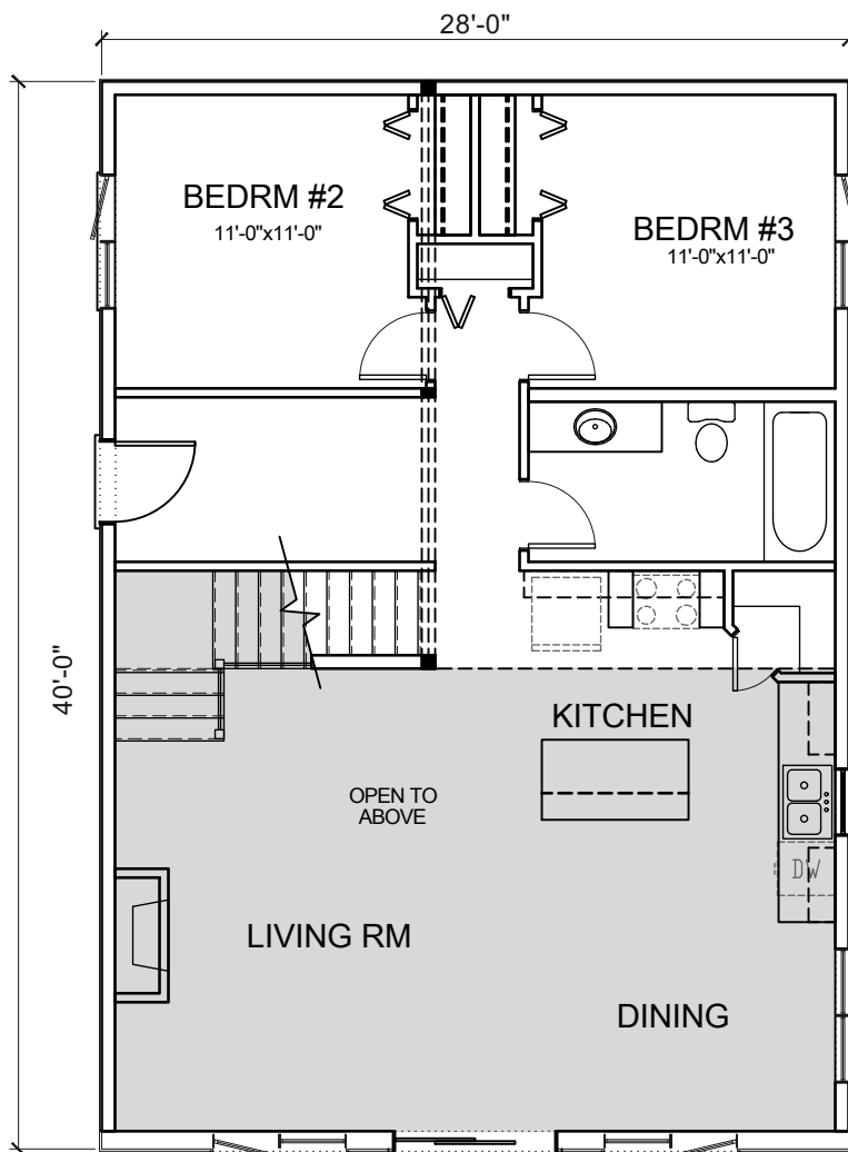
MAIN FLOOR PLAN #1615 1120 SQ. FT.
