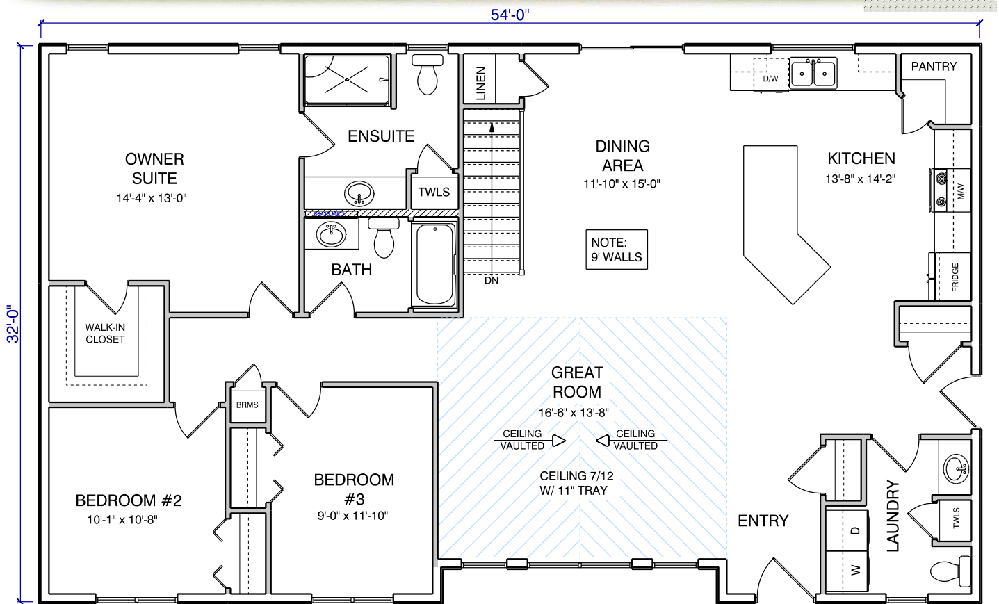
FLOOR PLAN #1600 1696 SQ. FT.
