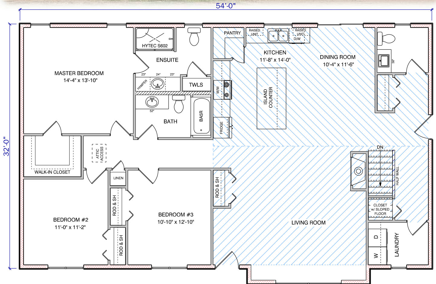
FLOOR PLAN #1705 1760 SQ. FT.
