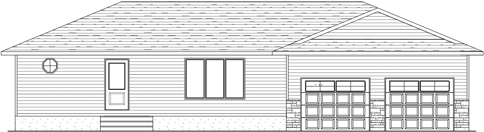
FRONT ELEVATION
