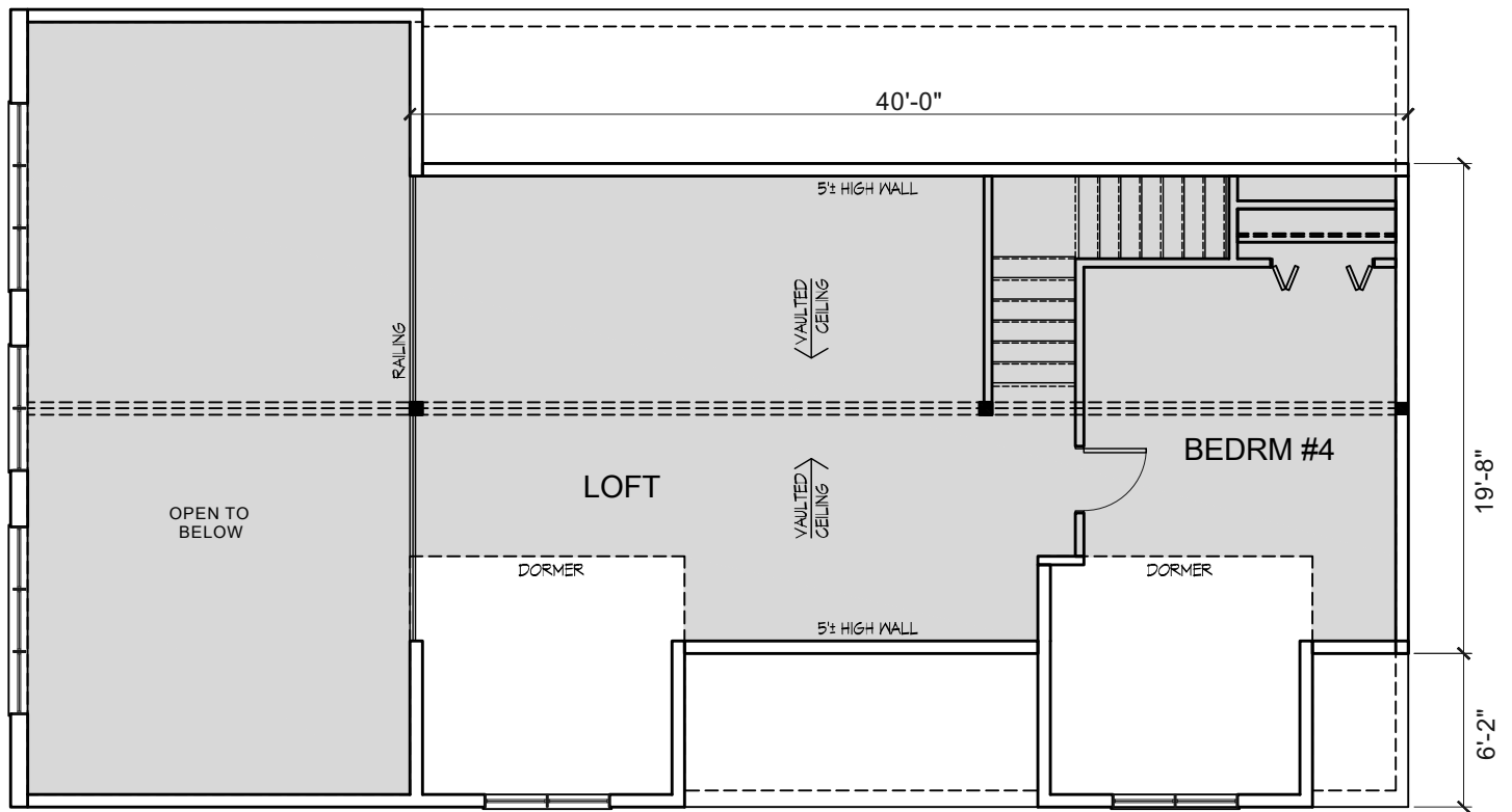
UPPER FLOOR PLAN #2600 866 SQ. FT. + STAIRS
