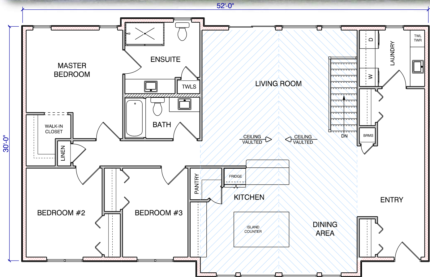
FLOOR PLAN #1613 1613 SQ. FT.
