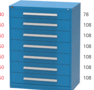
RP3512AL 59 in. (1499 mm) High 7 Drawers 208 Compartments Usable Drawer Heights 5-3/8 in. (137 mm) 7 in. (178 mm) 893 lbs. (405 kg.) Shipping Weight
