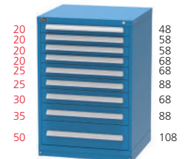
SEP2025AL 9 Drawers 184 Compartments Usable Drawer Heights 2-1/4 in. (57 mm) 3 in. (76 mm) 3-7/8 in. (98 mm) 4-5/8 in. (117 mm) 7 in. (178 mm) 485 lbs. (220 kg.) Shipping Weight
