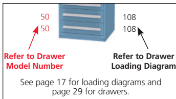
SCU1910AL 6 Drawers 144 Compartments Usable Drawer Heights 3-7/8 in. (98 mm) 5-3/8 in. (137 mm) 379 lbs. (172 kg.) Shipping Weight
