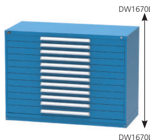
RP2149AL 44 in. (1118 mm) High 12 Drawers 24 Compartments Usable Drawer Heights 2-1/4 in. (57 mm) 3 in. (76 mm) 905 lbs. (411 kg.) Shipping Weight
