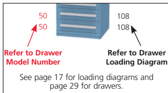
SCU1004AL 6 Drawers 124 Compartments Usable Drawer Heights 2-1/4 in. (57 mm) 3 in. (76 mm) 3-7/8 in. (98 mm) 7 in. (178 mm) 385 lbs. (175 kg.) Shipping Weight
