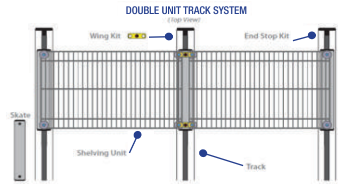
DOUBLE DEEP FLOOR TRACK ASSEMBLES
