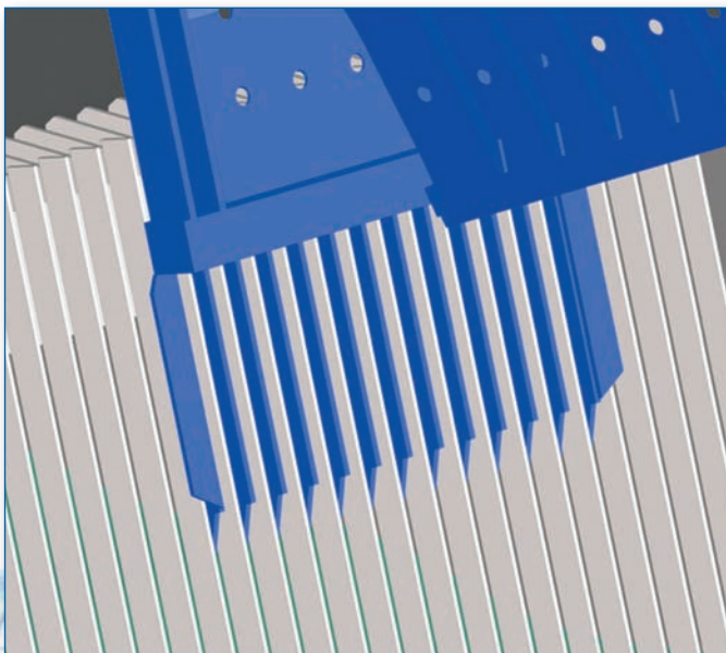
The prongs of the grab penetrate deeply into the screen
