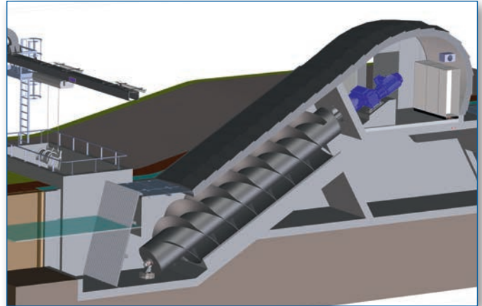
LANDY screen cleaner with Archimedes screw pump
