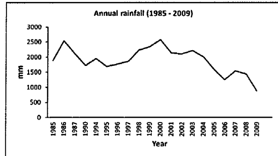
Figure 1. Annual rainfall (1985-2009) in Nuwakot, Nepal.
