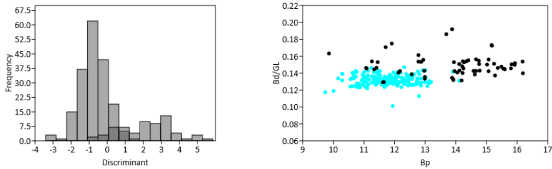
Figure 2.6: Results of the analysis of radius measurements Bp and Bd/GL. Left - result of the DA with the dark grey highlighting overlap. Right - scatter plot demonstrating a small degree of overlap between foxes (blue) and dogs (black).
