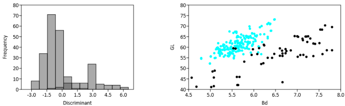
Figure 2.5: Results of the analyses of the four metapodials measurements Bd and GL. Left side - results of the DA with the dark grey highlighting overlap between the two species. Right side - scatter plots demonstrating varying degrees of overlap between foxes (blue) and dogs (black).
