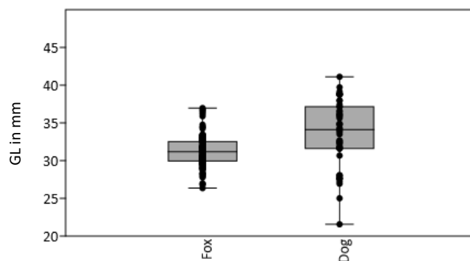
Figure 2.2: Box plot comparing the calcaneus GL (in mm) of foxes and dogs.
