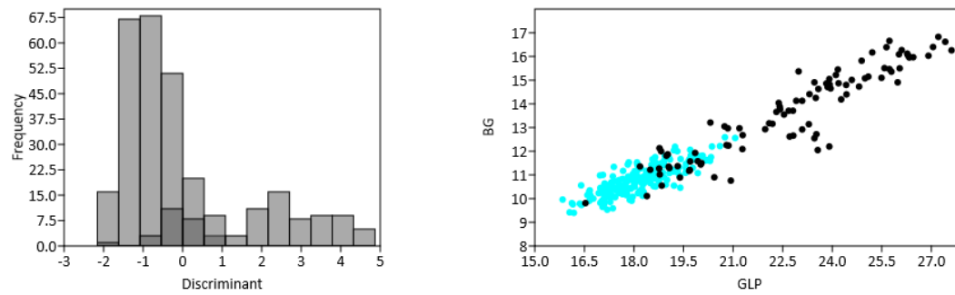
Figure 2.7: Results of the analysis of scapula measurements GLP and BG. Left - result of the DA with the dark grey highlighting overlap. Right - scatter plot demonstrating some degree of overlap between foxes (blue) and dogs (black).
