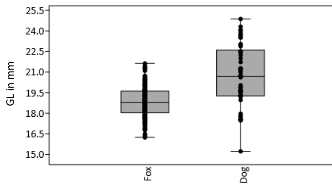
Figure 2.1: Box plot comparing the astragalus GL (in mm) of foxes and dogs.
