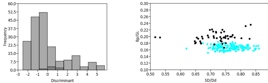
Figure 2.8: Results of the analysis of tibia measurements SD/Dd and Bp/GL. Left - result of the DA with the dark grey highlighting overlap. Right - scatter plot demonstrating only a small degree of overlap between foxes (blue) and dogs (black).
