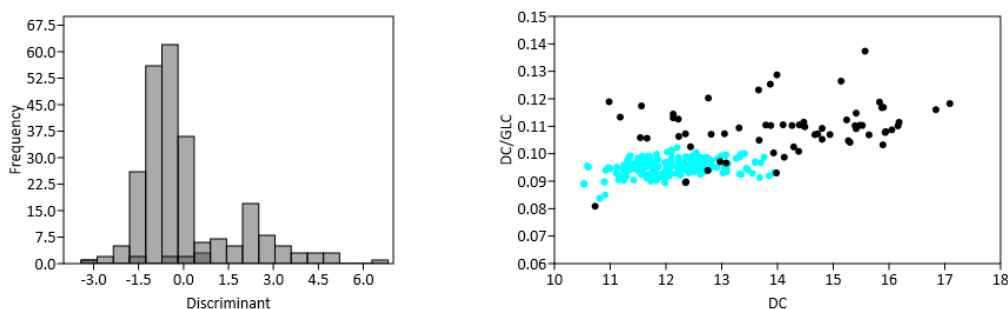
Figure 2.3: Results of the analysis of femur measurements DC and DC/GLC. Left - result of the DA with the dark grey highlighting overlap. Right - scatter plot demonstrating a small degree of overlap between foxes (blue) and dogs (black).
