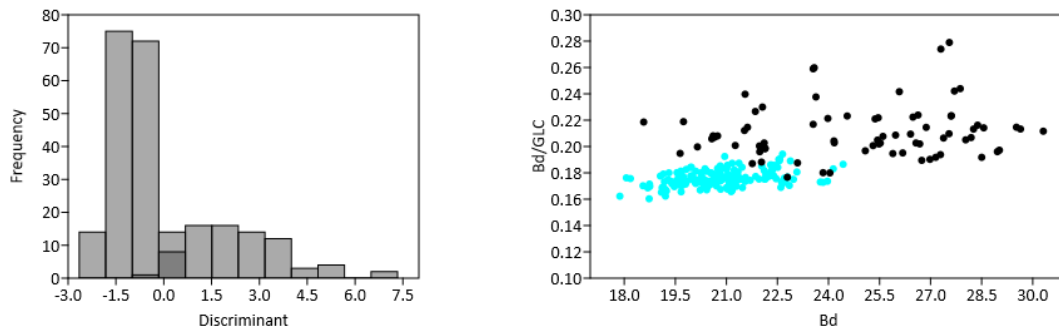
Figure 2.4: Results of the analysis of humerus measurements Bd and Bd/GLC. Left - result of the DA with the dark grey highlighting overlap. Right - scatter plot demonstrating a small degree of overlap between foxes (blue) and dogs (black).
