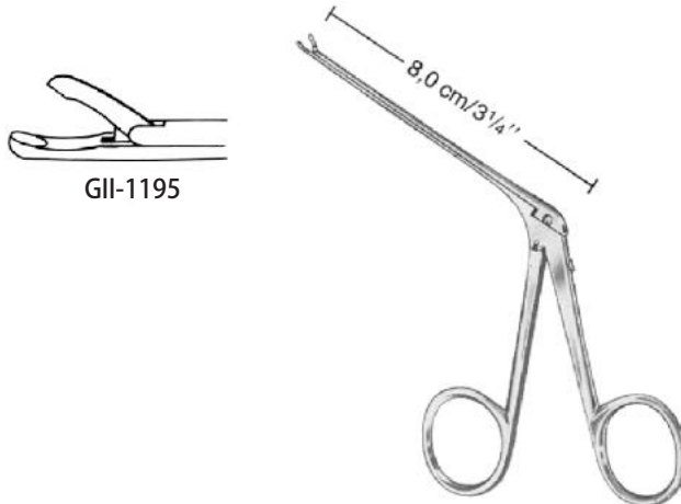
Crura-Nipper Micro Ear Forceps
