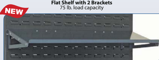
SLP-A1236 and SLP-A1836 Slanted Shelf with 2 Slanted Brackets 75 lb. load capacity
