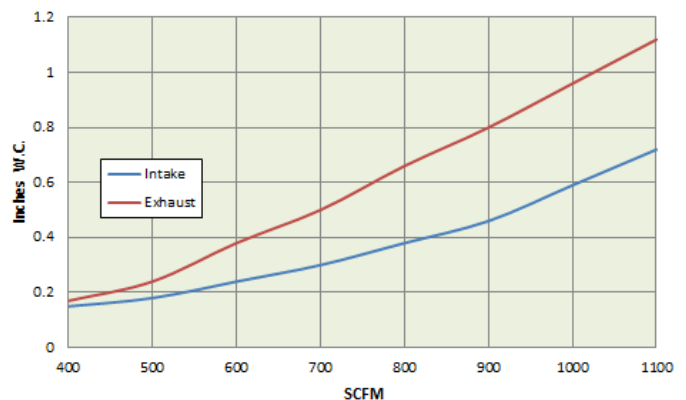
Flow Range Pressure Drop
