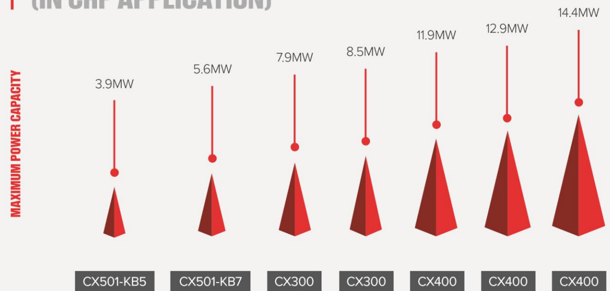
GENERATOR PACKAGE MODEL
