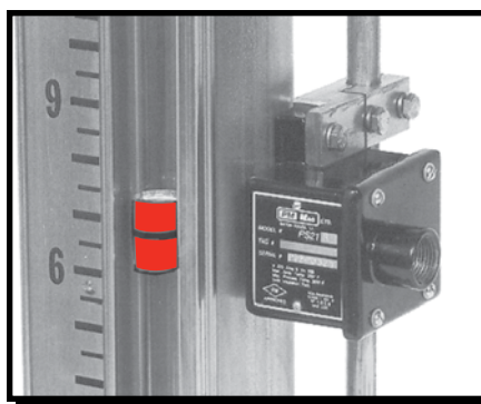
ES21 NEMA 4x ( Rod Mounted )
