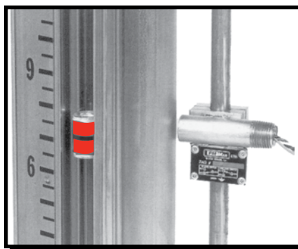
ES30EX Switch ( Rod Mounted )
