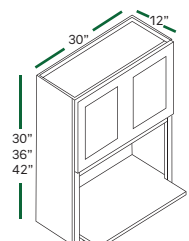
WALL MICROWAVE WM3030 WM3036 WM3042
