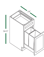
BASE WASTE BASKET B18TR
