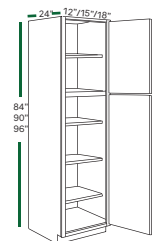
PANTRY 2 DOORS TP128424 TP129024 TP129624 TP158424 TP159024 TP159624 TP188424 TP189024 TP189624
