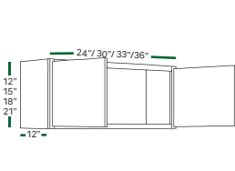
2 DOORS W3012 W2415 W2418 W3021 W3312 W3015 W3018 W3612 W3315 W3318 W3615 W3618
