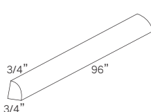
QUARTER ROUND MOLDING QRM
