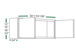
2 DOORS W301224 W301524 W301824 W302424 W331224 W331824 W332424 W361224 W361824 W362424
