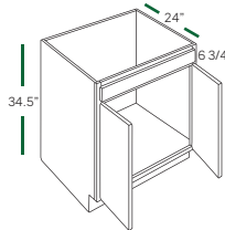
SINK BASE SB24 SB30 SB36 SB27 SB33
