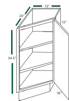
TRANSITIONAL BASE BTR12 BTL12
