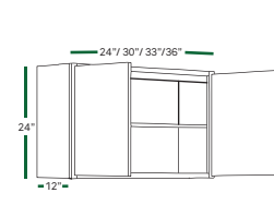
2 DOORS W2424 W3024 W3324 W3624
