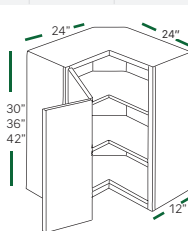
PIE CUT CORNER WPC2430 WPC2436 WPC2442
