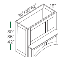
CUSTOM HOOD RHA3030 RHA4230 RHA3630 RHA4236 RHA4242
