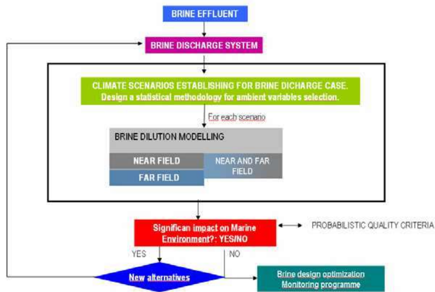
Fig. 6. Scheme of brine discharge modelling.
