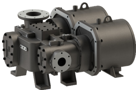
Dual air end and dual motor connection in series
