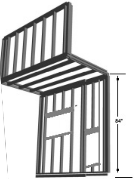
EXTERIOR TONGUE FRAMING VIEW
