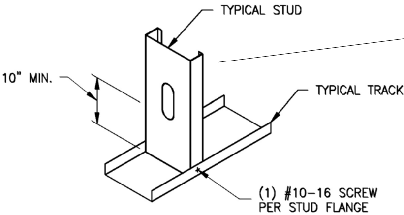
STUD TO TRACK ATTACHMENT
