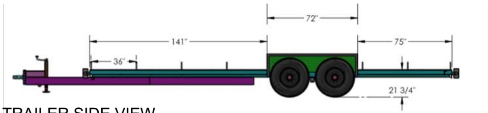
TRAILER SIDE VIEW
