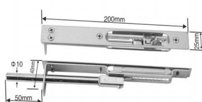
Model: HFX002 (8-inch special safety pin insertion) Size: 200X25X40mm
