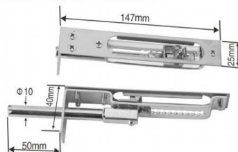
Model: HFX001 (6-inch special safety pin insertion) Size: 147X25X40mm
