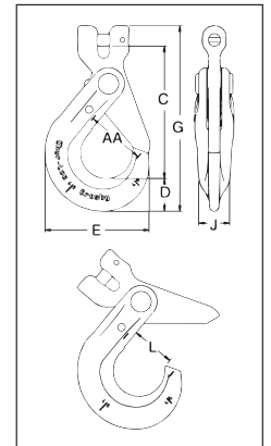
S-1317 Clevis Hook
