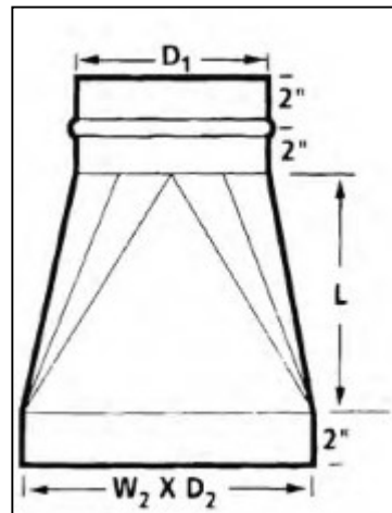
SQ 2RD SQUARE/OVAL TO ROUND
