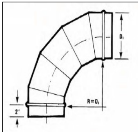
DC - 90 90° GORE LOCKED ELBOW R = 1.5 \times D
