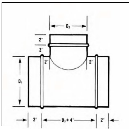
DCT - 90 90° TEE
