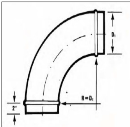
DC - 90 90° DIE STAMPED ELBOW R = 1.5 \times D
