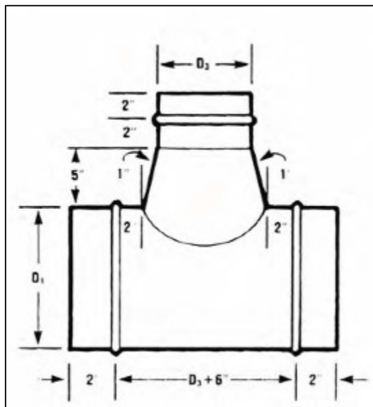
DCCT - 90 90° CONICAL TEE
