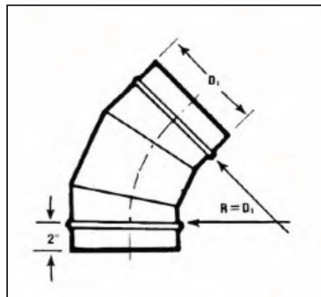
DC - 45 45° GORE LOCKED ELBOW R = 1.5 \times D
