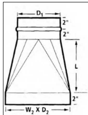
SQ 2RD SQUARE TO ROUND
