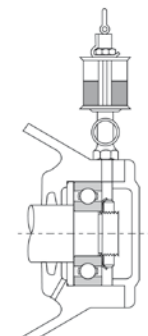
Drip Feed Lubrication: for high speeds
