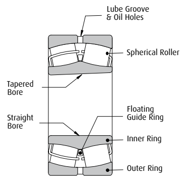
Spherical Roller Bearing
