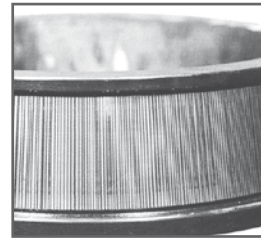
Electrical Corrosion
