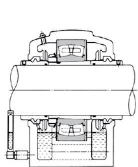
Oil Bath Lubrication: not for high speeds
