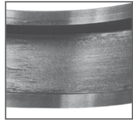
Smearing
