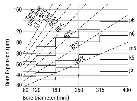
Figure 1: Temperature and Expansion of Inner Ring
