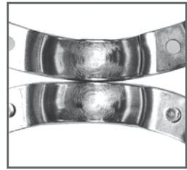
Scoring
