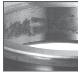
Fretting
