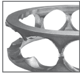
Cage Damage
