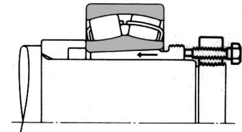
Mounting with Withdrawal Sleeve
