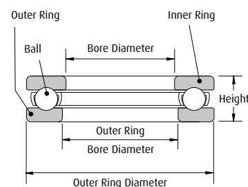
Single Direction Thrust Ball Bearing
