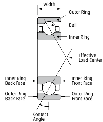
Single Row Angular Contact Ball Bearing
