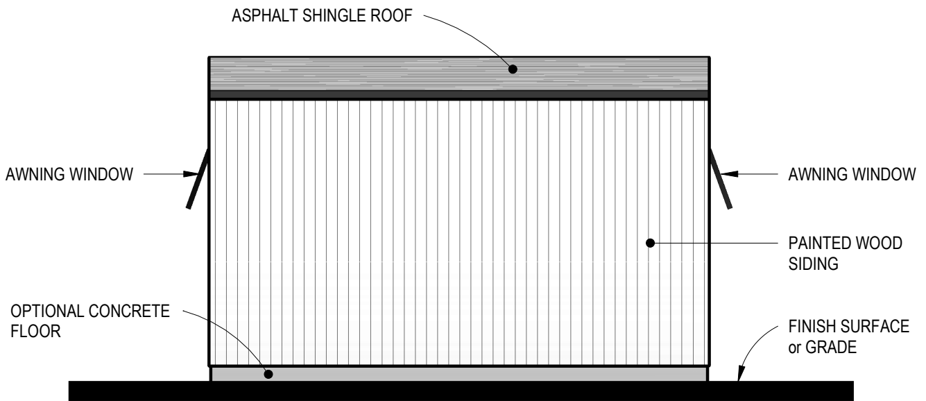
REAR ELEVATION
