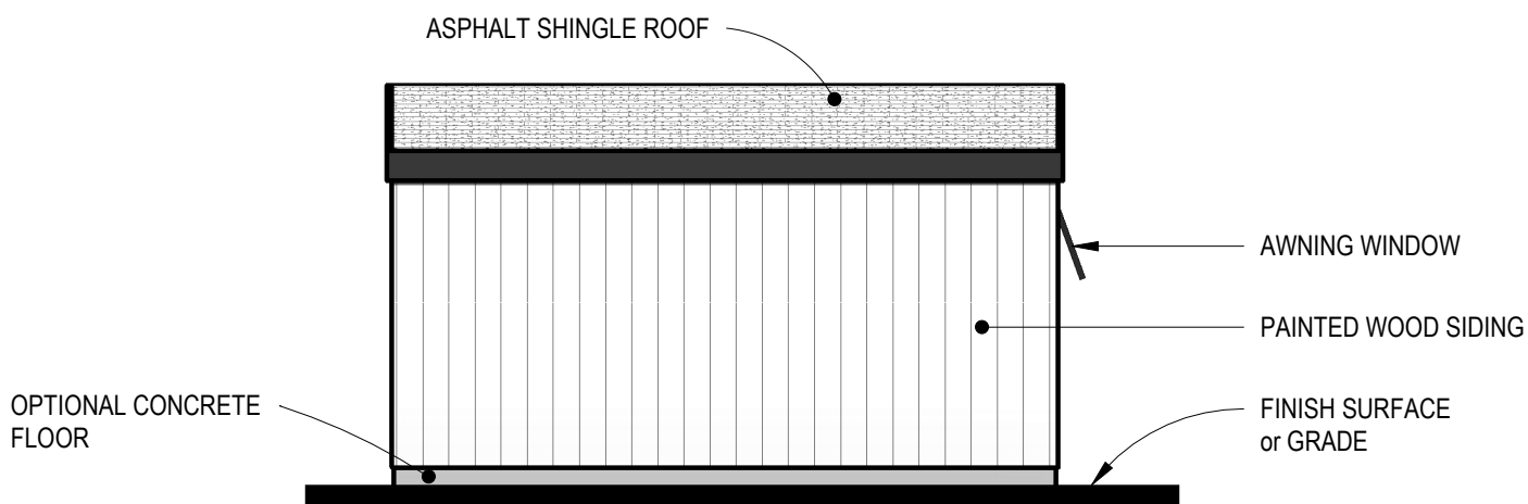
REAR ELEVATION
