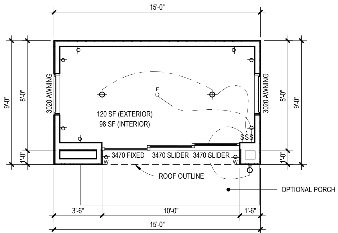
FLOOR PLAN
