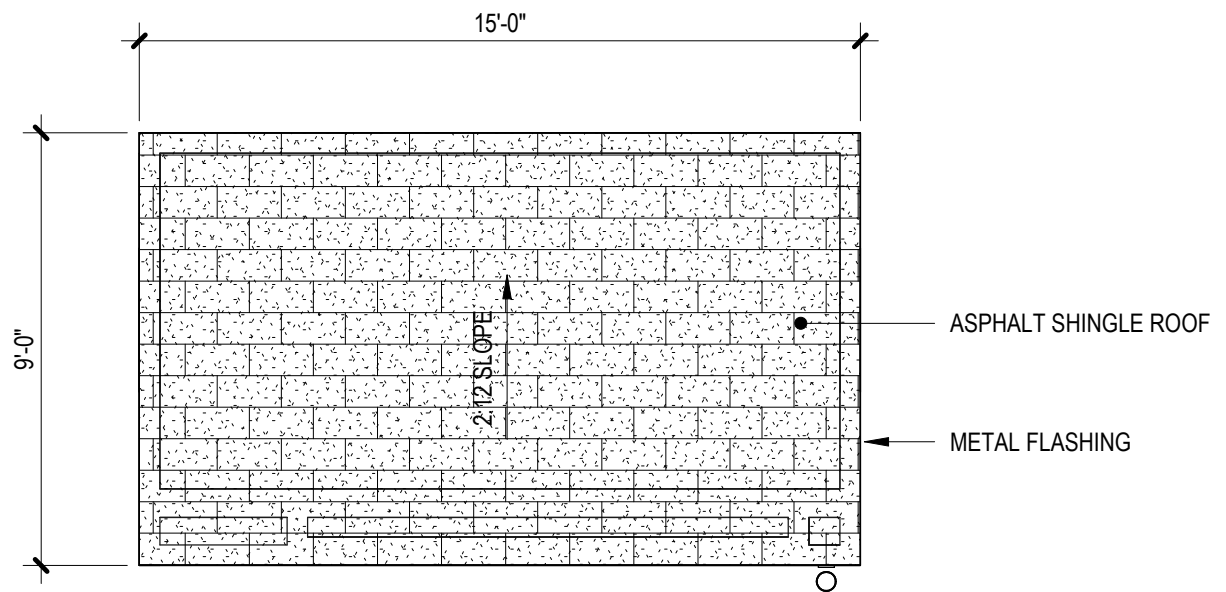
ROOF PLAN
