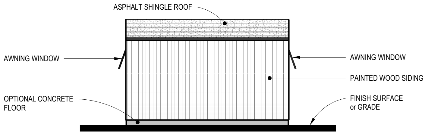
REAR ELEVATION
