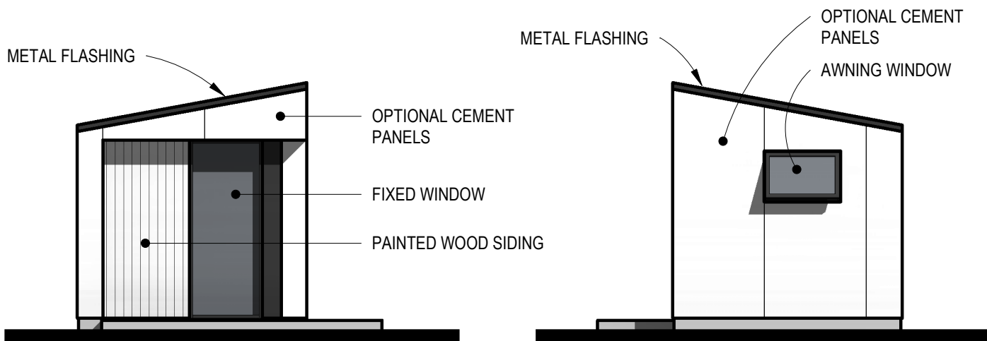
LEFT ELEVATION
