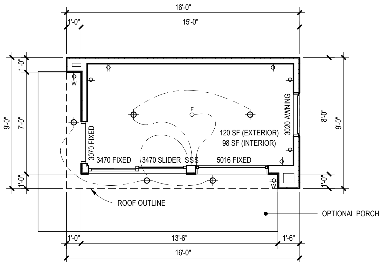
FLOOR PLAN
