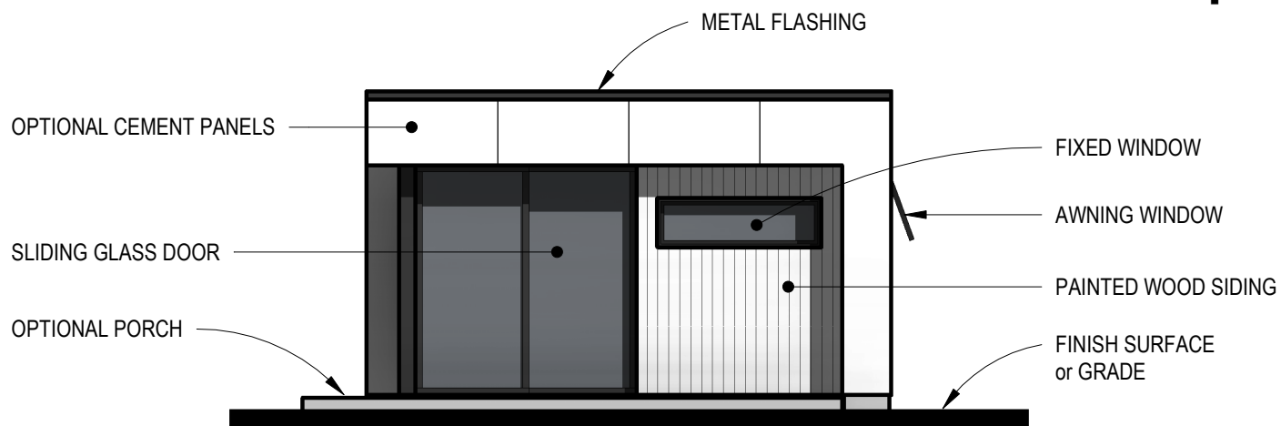
FRONT ELEVATION
