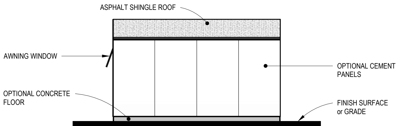
REAR ELEVATION
