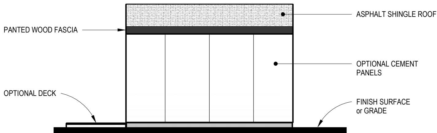
REAR ELEVATION
