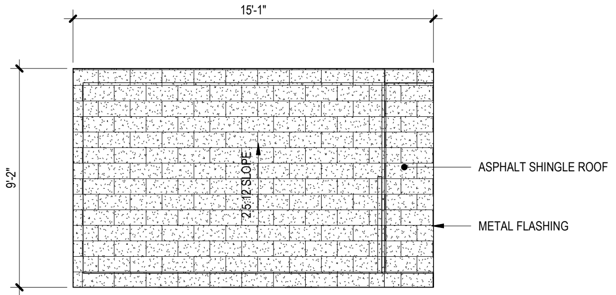
ROOF PLAN
