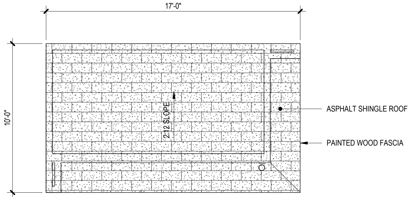
ROOF PLAN
