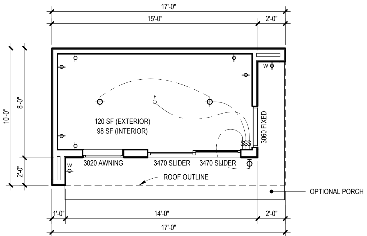
FLOOR PLAN
