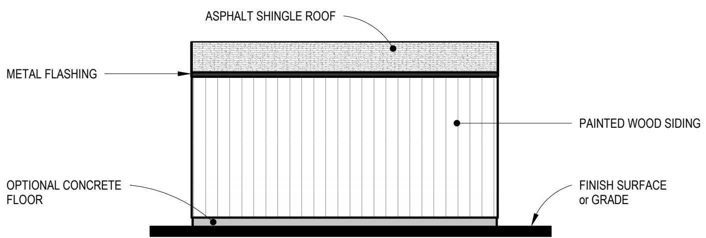
REAR ELEVATION
