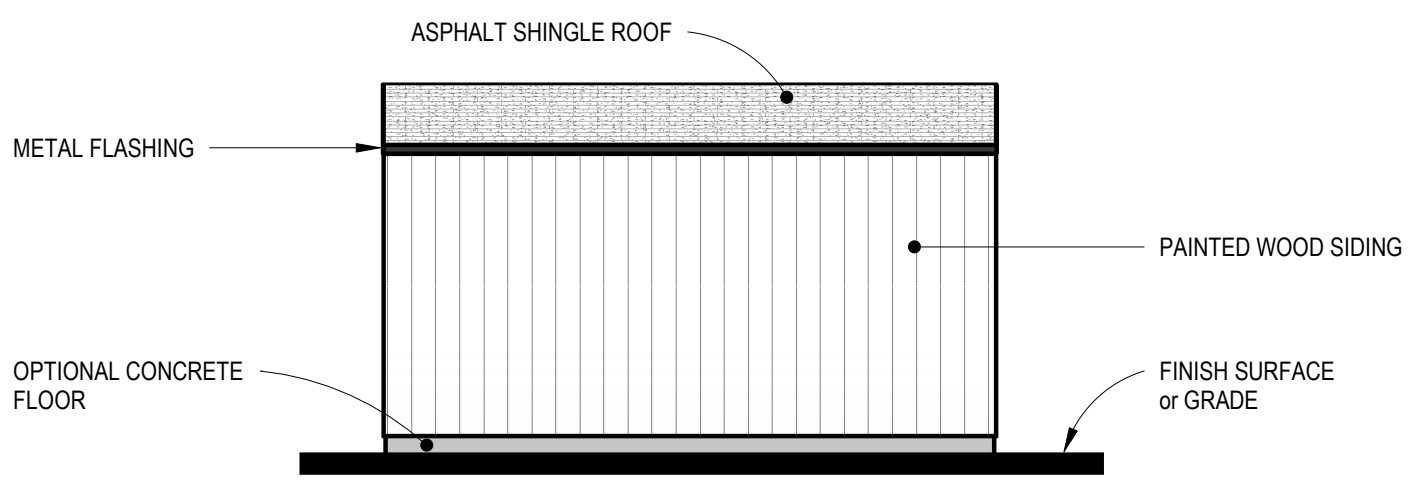
REAR ELEVATION
