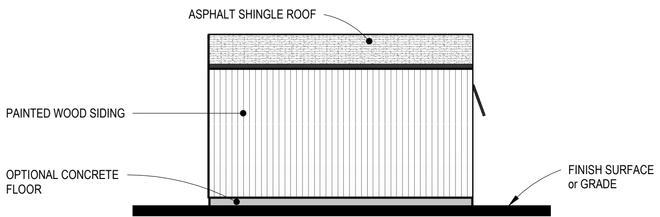
REAR ELEVATION
