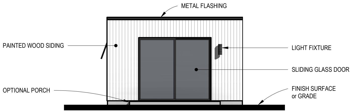
FRONT ELEVATION
