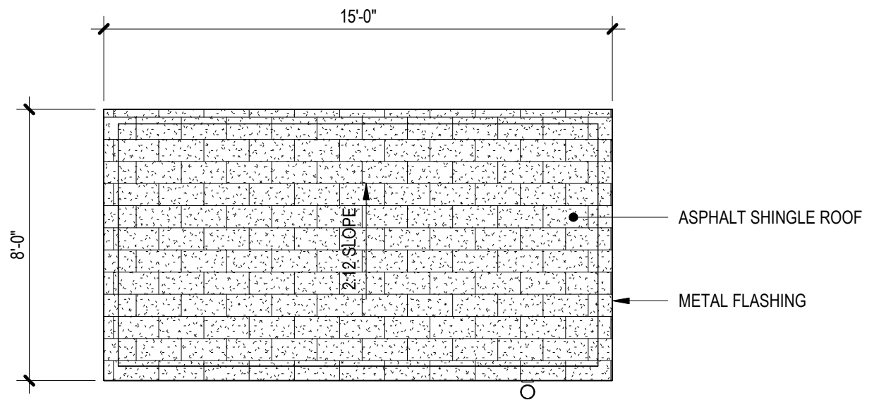
ROOF PLAN
