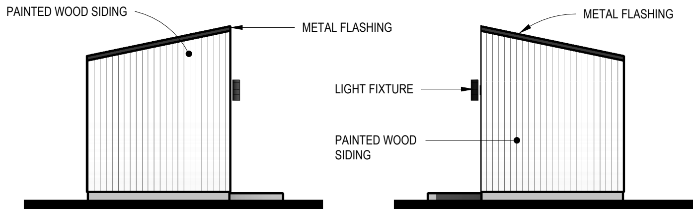
LEFT ELEVATION
