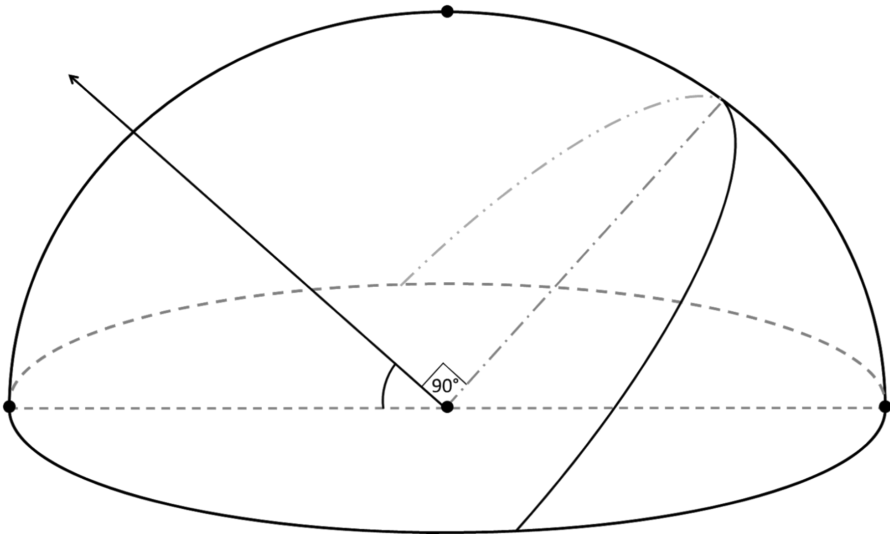
Celestial Sphere
