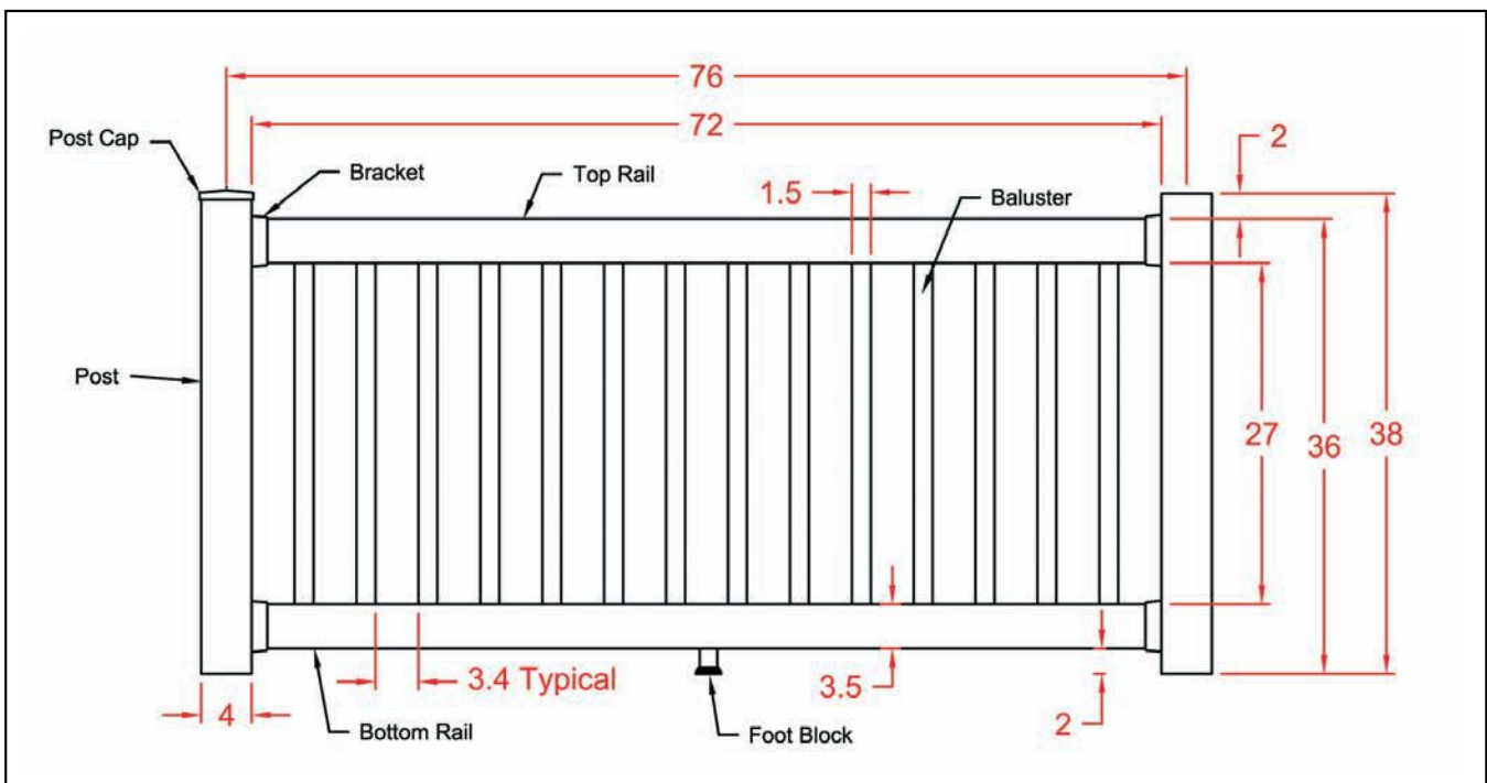
Shop drawing shown for 36" (H) x 72" (L) level railing kit. Other drawings available upon request.
