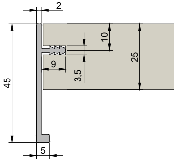
HAND20 - MANIGLIA HANDLE P10525
