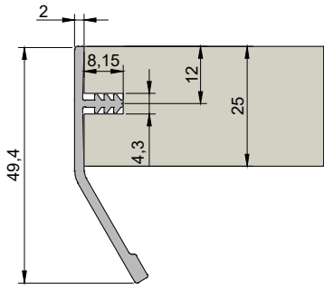
HAND16 - MANIGLIA HANDLE P10262
