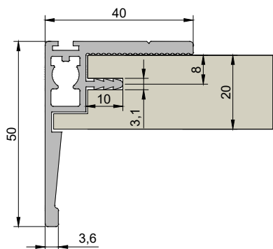
HAND14 - MANIGLIA HANDLE P10316
