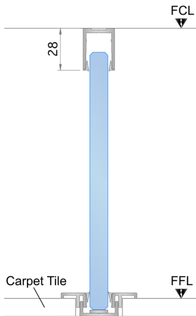
Solo Head & Base Detail
