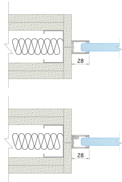
Solo abutment details
