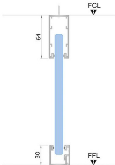
cristal deflection head detail
