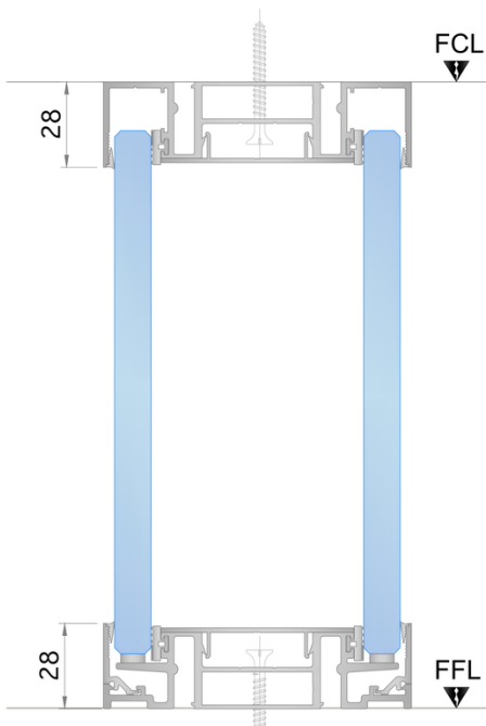
Asteria Head & Base Detail
