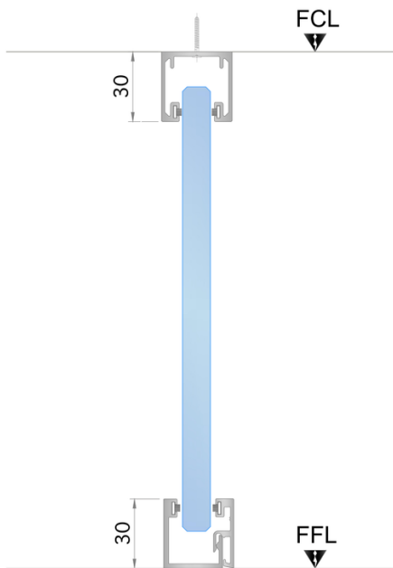
Cristal Head & Base Detail
