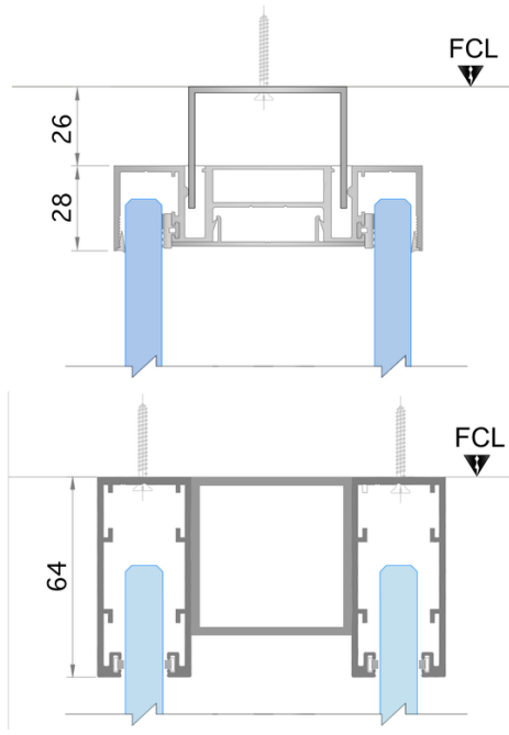
Asteria deflection head detail
