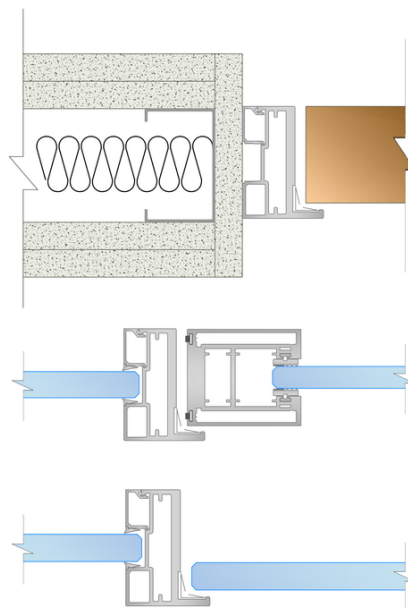
Klariti frame integrated with timber, mirage sg and frameless glass doors
