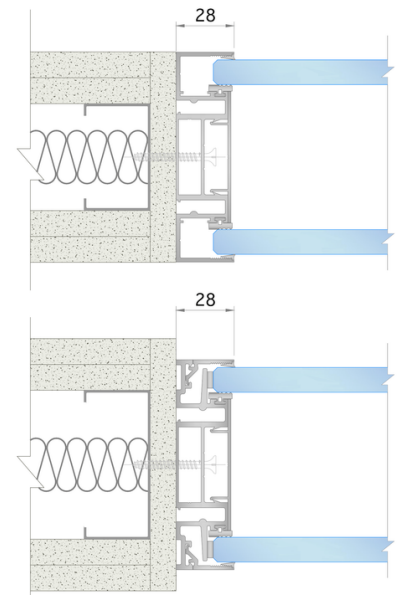
Asteria abutment details
