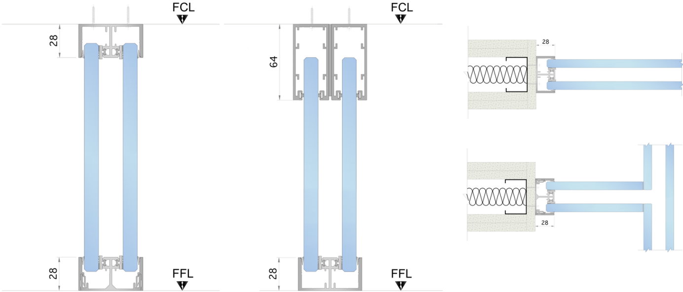
Neo Head & Base Detail
