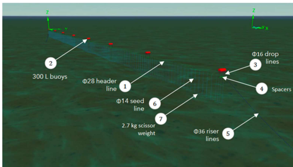
Figure 2: Arc Marine rendition of the seaweed farm longline structure
