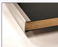
Plywood core with Laminate top and Channel Aluminum Edging
