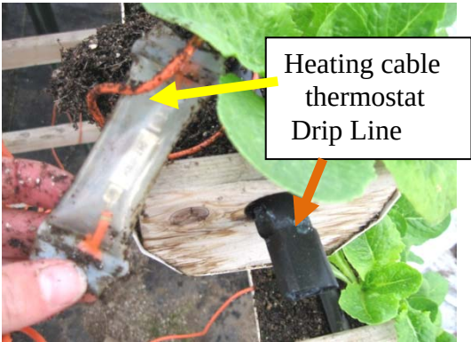
prevent the soil media from freezing and to promote Figure 5. Soil heating cable used in PVC gutter.
