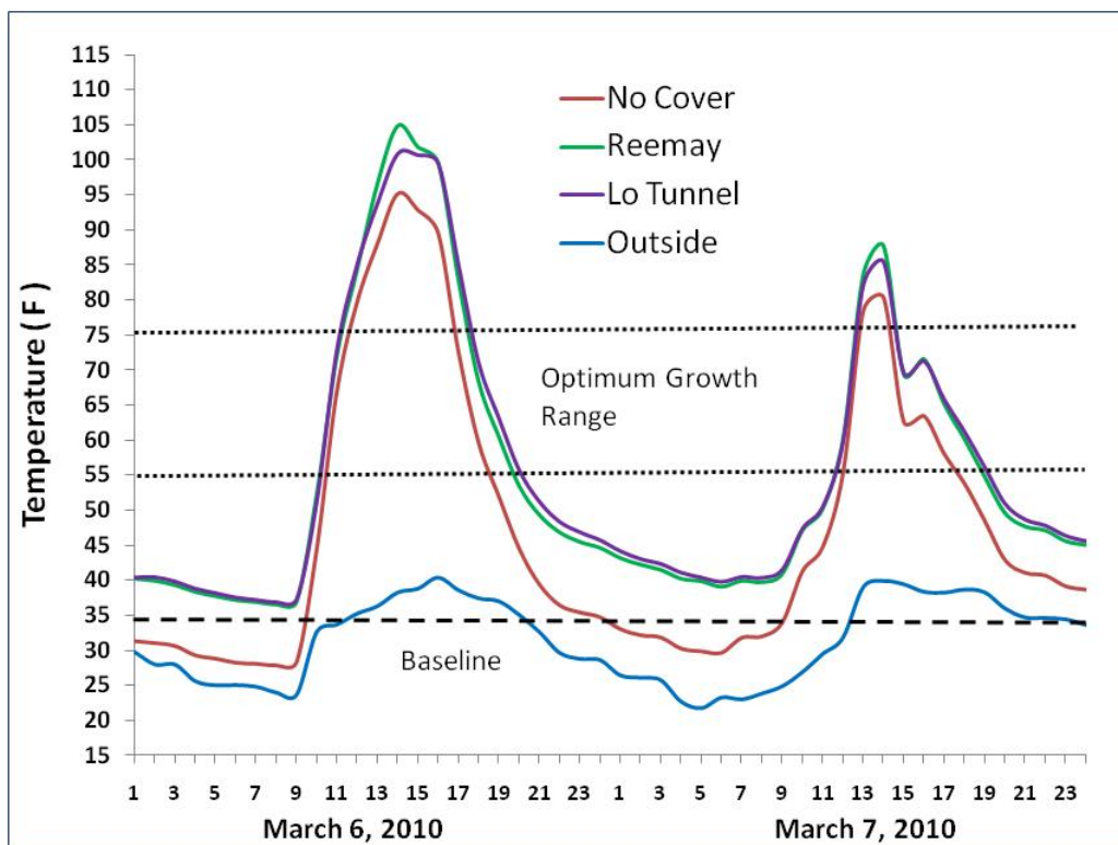
Figure 1. The change in hourly mean air temperature outside and under various row covers (Reemay, Lo Tunnel) in a high tunnel over 2 days in early March 2010.
