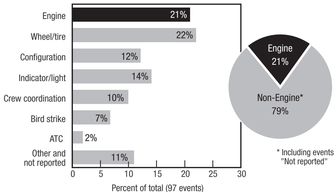
Figure 5 Reasons for initiating the RTO (97 accidents/ incident events)
